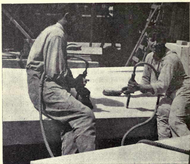
FIG. 79—USING PNEUMATIC TOOLS IN FINISHING CONCRETE
